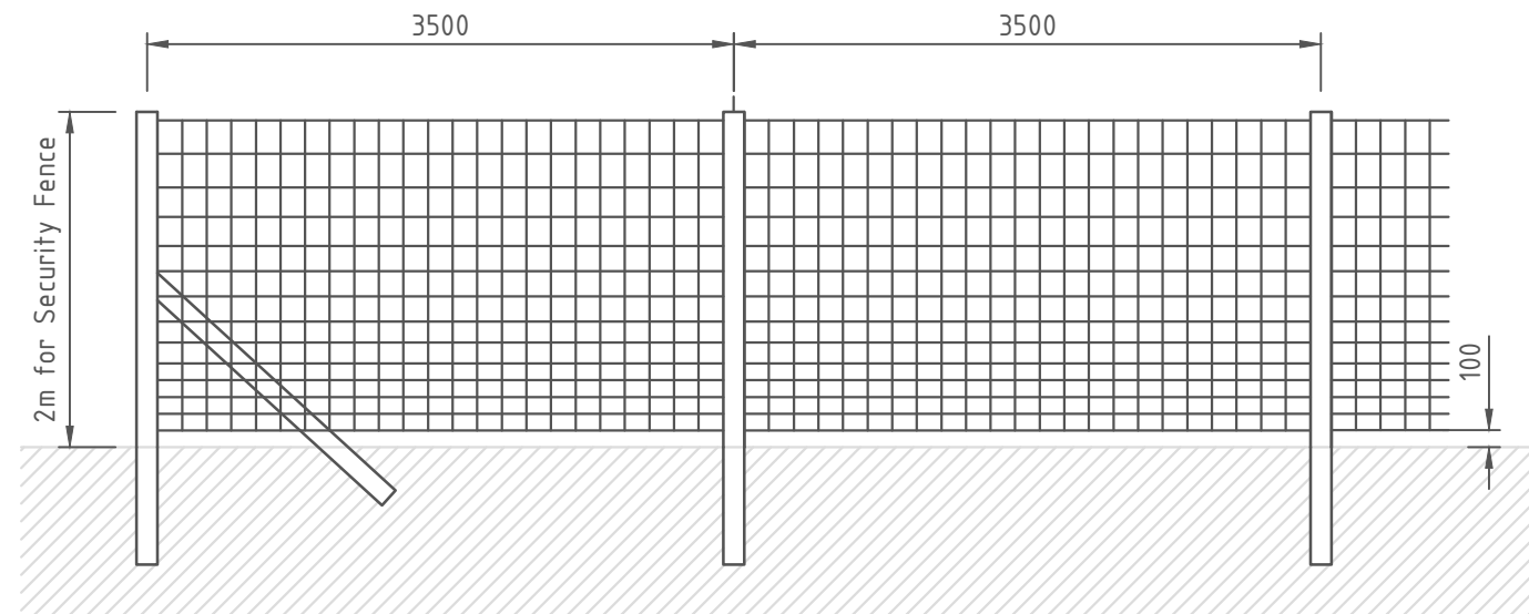
TYPICAL DEER FENCE ELEVATION
