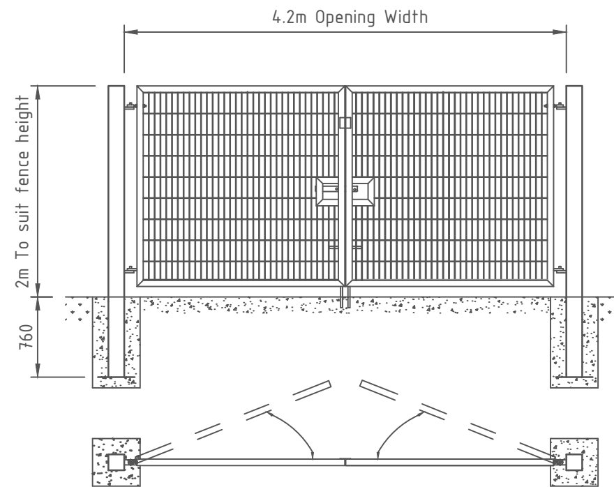
TYPICAL SECURITY GATE ELEVATION
